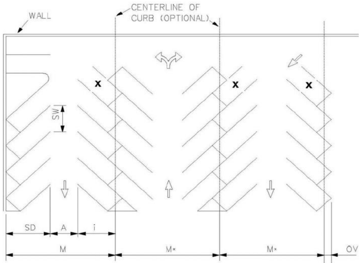
FIGURE 17 PARKING LAYOUT TERMS
