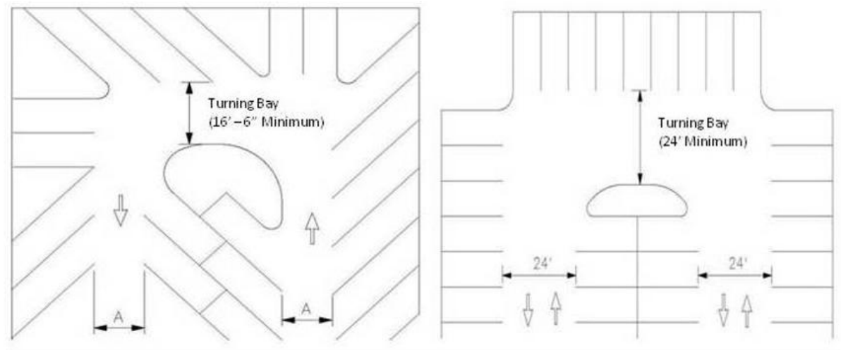
FIGURE 18. MINIMUM TURNING BAY DIMENSION FOR ONE-WAY AND TWO-WAY TRAFFIC FLOW
